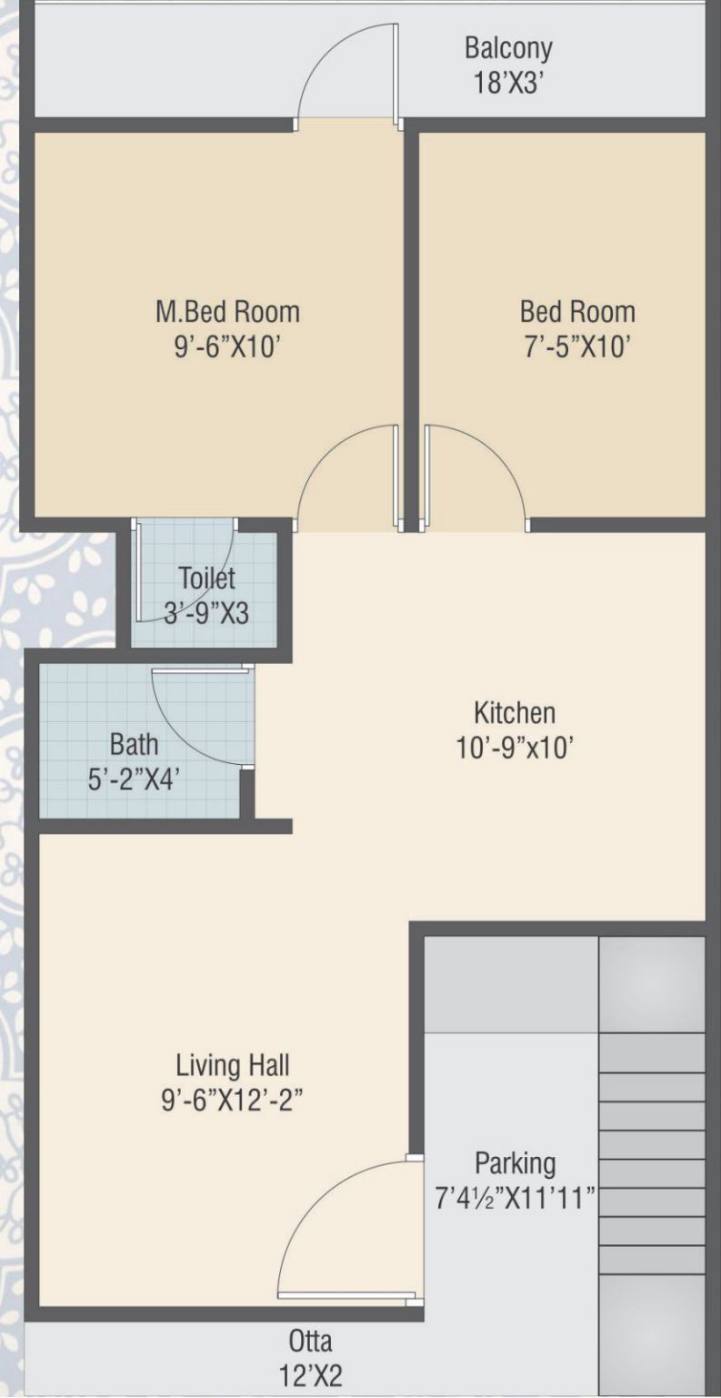
18X36 GROUND FLOOR PLAN
